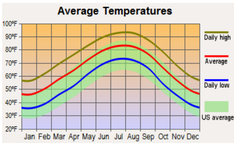
General temperatures for South Louisiana.
